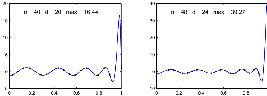
FIG. 3.1. Maximal polynomials p of degree n/2 on [-1, 1] for n = 40 and 48 subject to the constraint |p(x_j)| \leq 1 on the equispaced n -grid. (The polynomials are even, and only the right half of the interval is shown.) As shown by Coppersmith and Rivlin [9], the maximum grows exponentially as n \rightarrow \infty , and this observation is a key step in the proof of Theorems 1 and 2.
