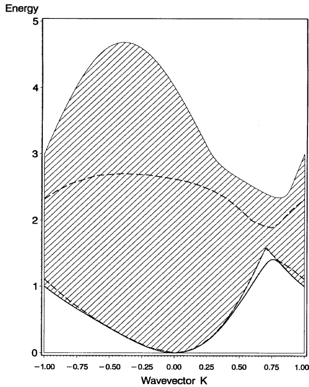
Figure 2. The two-magnon excitation spectrum showing the bound-state branch (solid line), the scattering-state continuum (shaded region) and the resonances (dashed lines) for the S = 1 Tsvetik model with \gamma = \frac{1}{2} . The energy is in units of 2SJ_1 and the wavevector K is in units of \pi/a .
