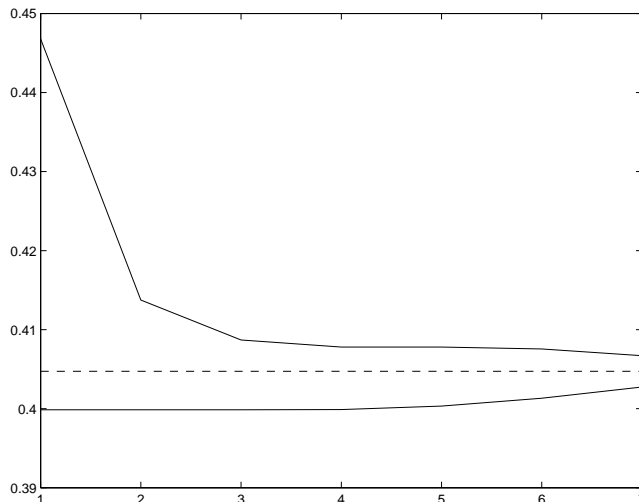
FIGURE 1. European options. Model 1
