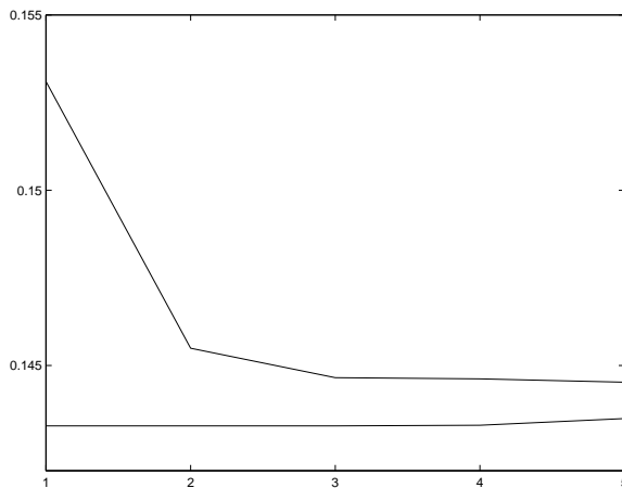
FIGURE 2. European options. Model 3
